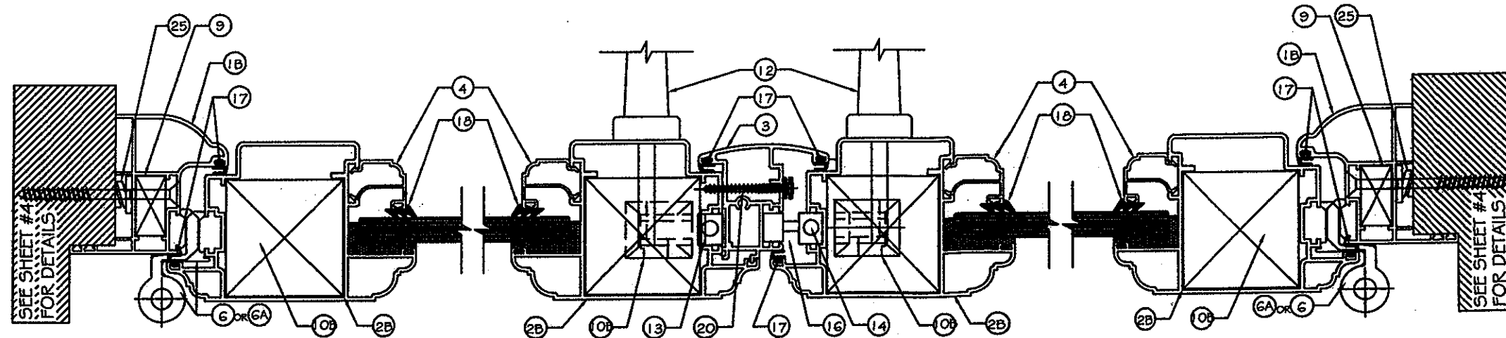
COMBINATION 4 SCALE: 3/16" = 1'-0"
