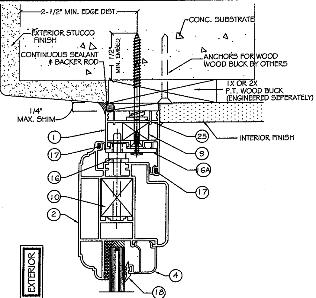
2 HEAD DETAIL (CONC. SUBSTRATE) 5 SCALE: 1/4" = 1'-0"
