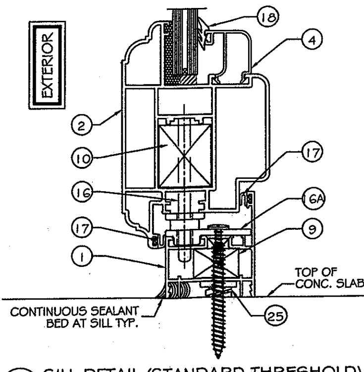
3 SILL DETAIL (STANDARD THRESHOLD) 5 SCALE: 1/4" = 1'-0"
