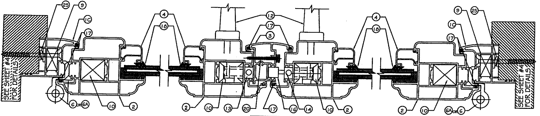
COMBINATION 2 SCALE: 3/16" = 1'-0"
