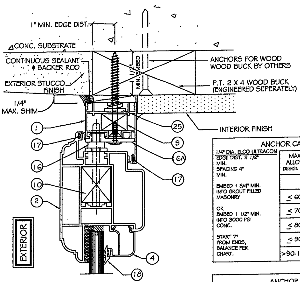
4 HEAD DETAIL (WOOD SUBSTRATE) 5 SCALE: 1/4" = 1'-0"
