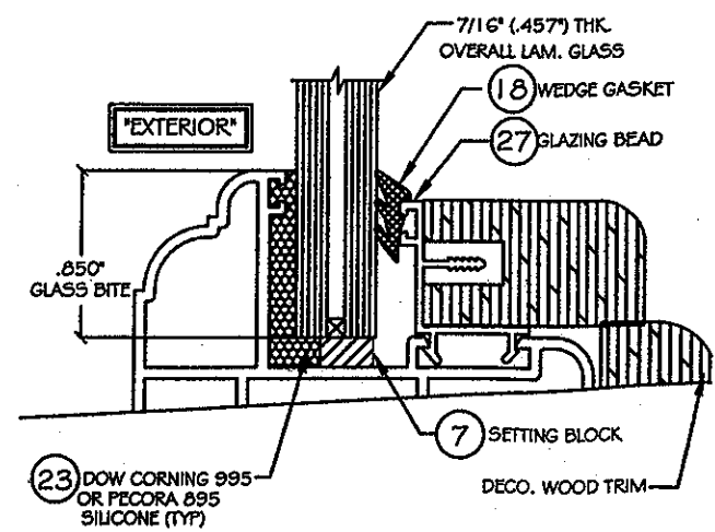
GLAZING DETAIL GL-1 (WITH WOOD TRIM) SCALE: NTS. OPTION MAX D.P. = +80 / -80 PSF
